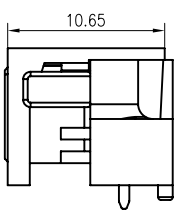
WITH CAP DRAWING SCALE:1:1
