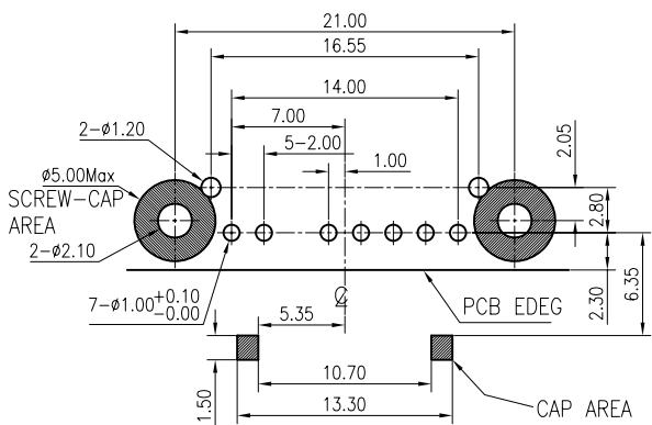
RECOMMENDED PCB LAYOUT(TOP VIEW) TOLERANCE±0.05mm,THICKNESS:1.20±0.05mm
